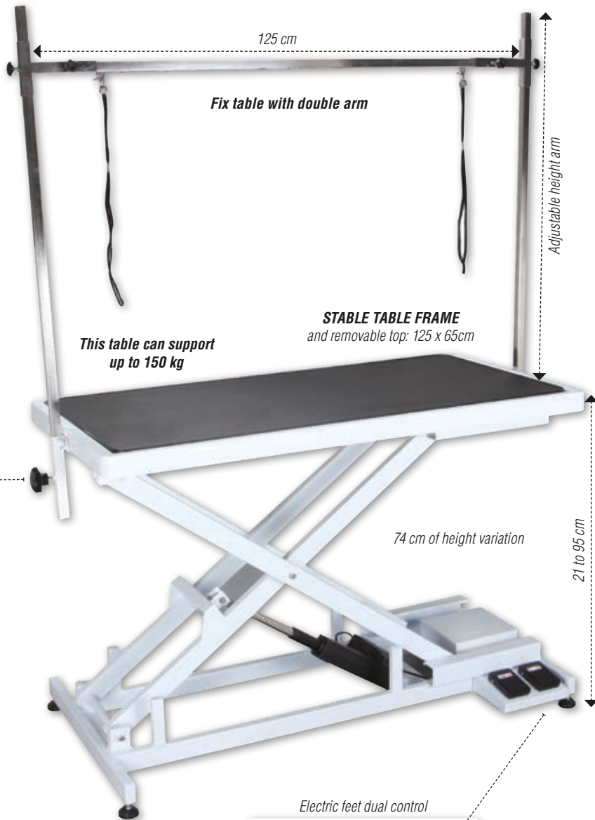
Adjustable arm
