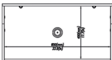
Draining hole
